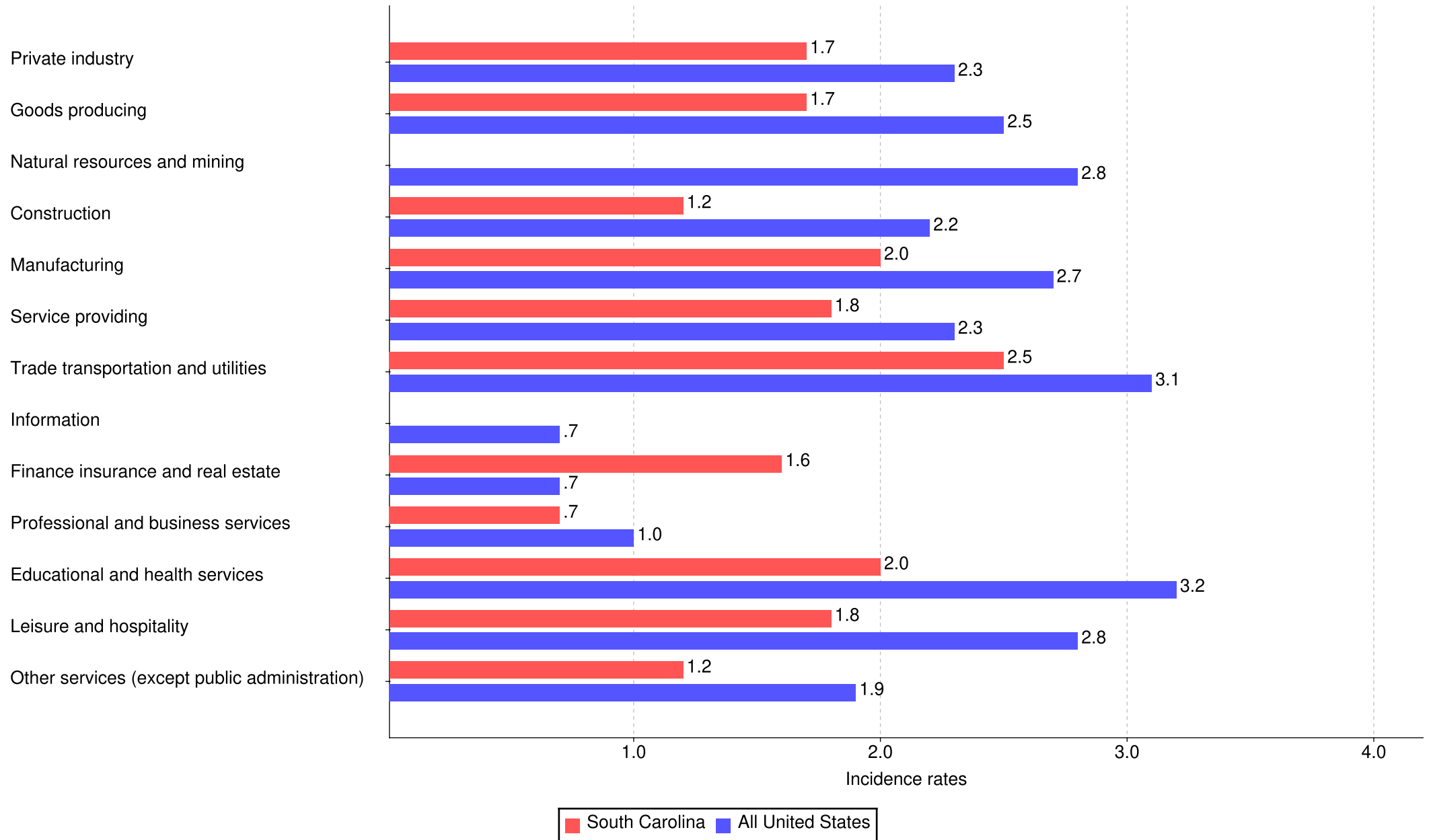
Incidence rates per 100 full-time workers for total nonfatal occupational injuries and illnesses by major industry sector, South Carolina and All United States, 2024
